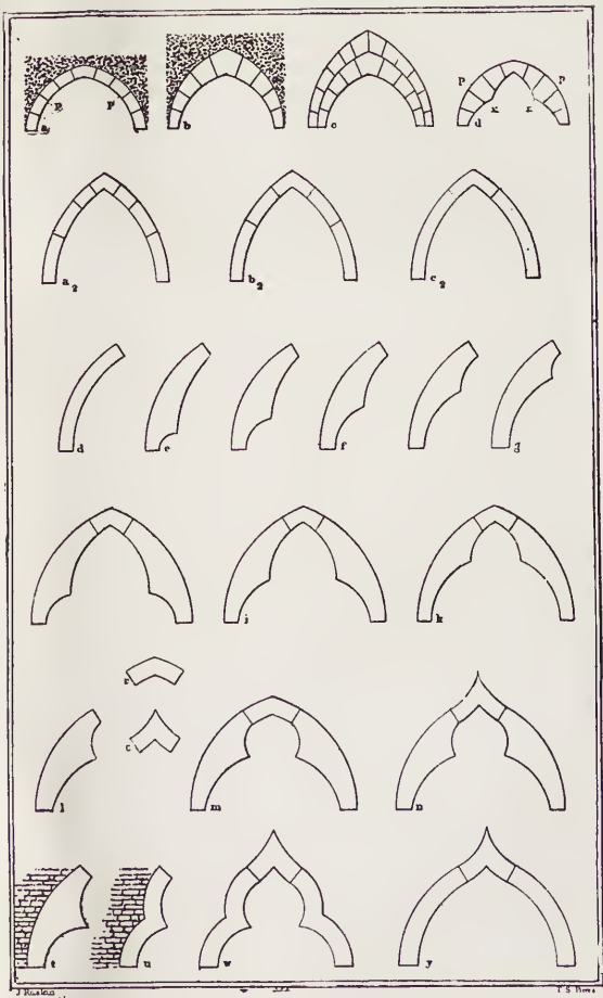
PLATE III: ARCH MASONRY
